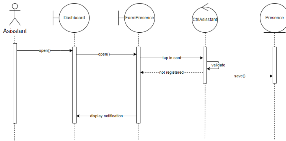
Figure 9. Process attendance
