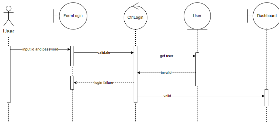
Figure 8. Admin Login
