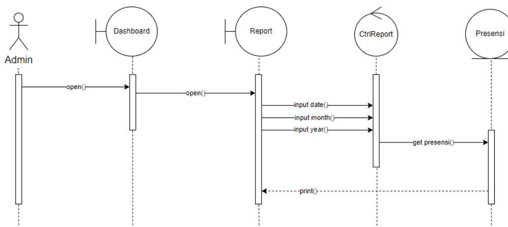
Figure 10. Report process
